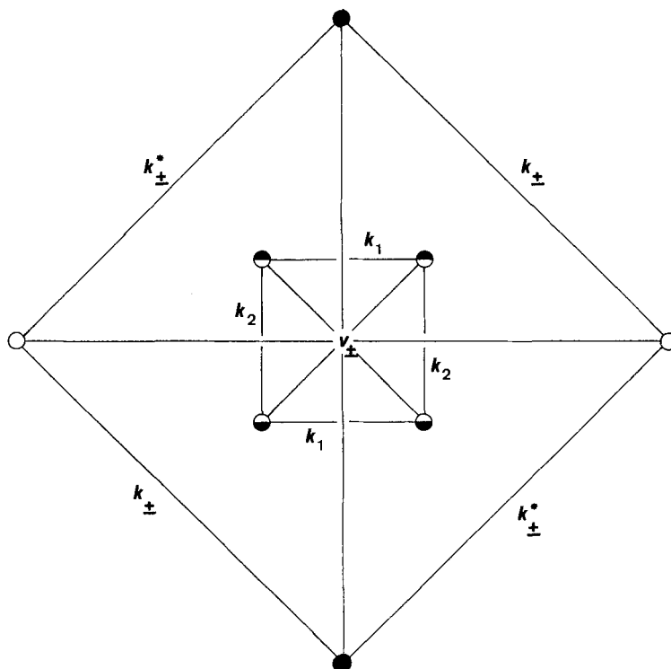
Fig. 13. Graph representation of all dynamic processes taking place in benzoocatalene 3 assuming that the interconversion 3c \rightleftharpoons 3b occurs via a \pi -bond shift in the octalene perimeter (i.e. via 3a ) (compare Fig. 12).
