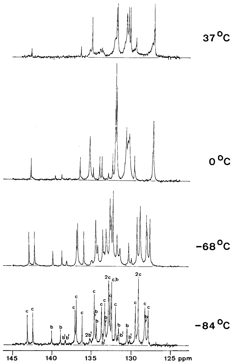
Fig. 4. ^1\text{H} -noise decoupled ^{13}\text{C} -NMR. spectra of benzoctalene 3 recorded at various temperatures (RF: 100.6 MHz)
