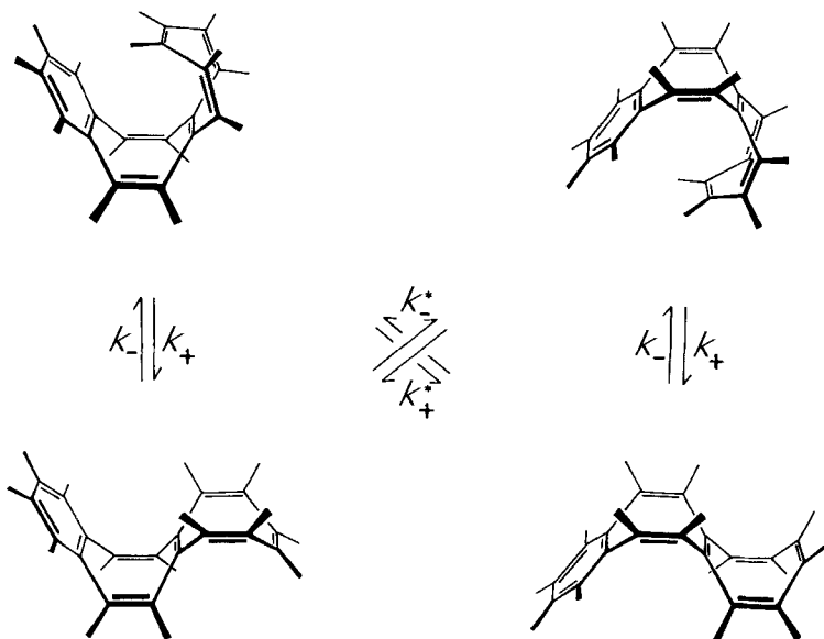
Fig. 7. Processes leading to interconversion of the conformers of benzo[8]octalene with double bond configuration 3b
