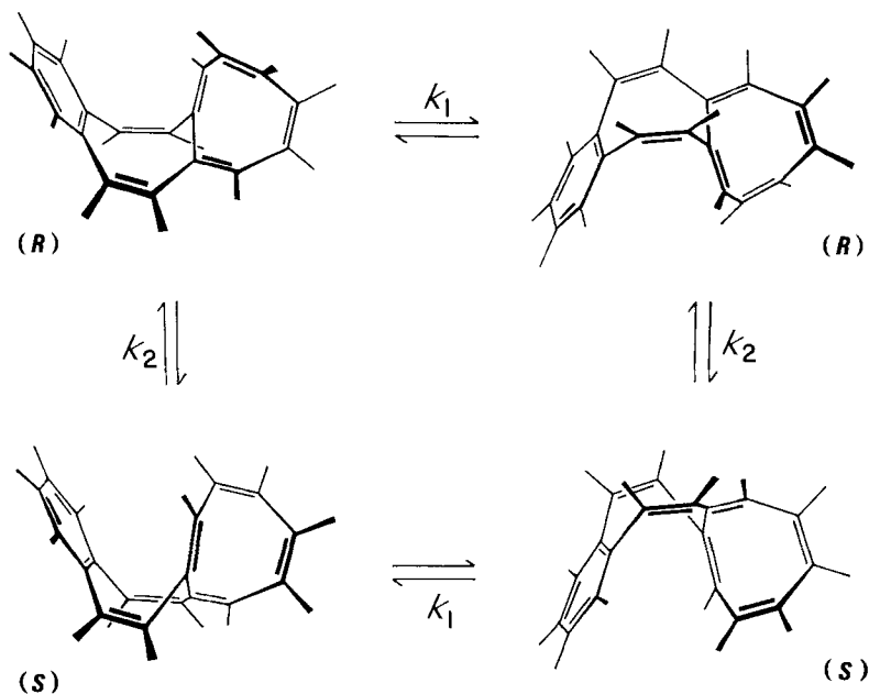
Fig. 5. Ring inversion processes in benzo[1,2-a:3,4-b']octalene with configuration 3c
