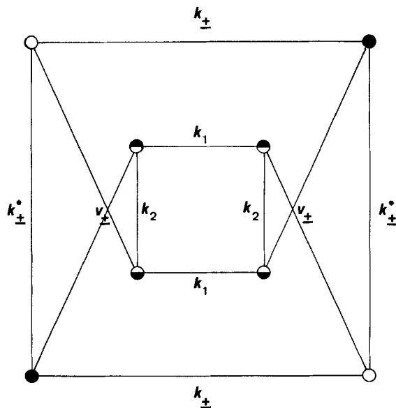
Fig. 12. Graph representation of all dynamic processes taking place in benzo[1,2-b:4,5-b']octalene 3 assuming that the interconversion \mathbf{3c} \rightleftharpoons \mathbf{3b} occurs via \pi -bond shift in the outer COT-ring (compare Fig. 5, 6 and 7).
